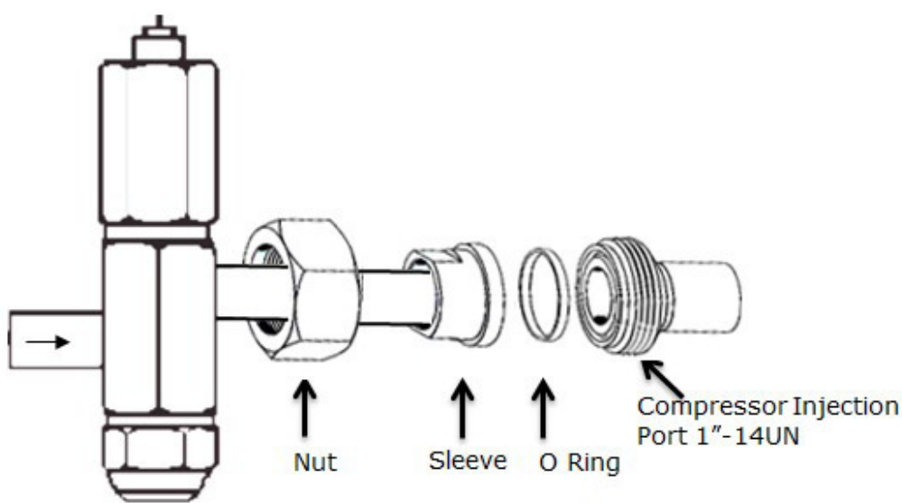
Figure A Rotolock fitting
