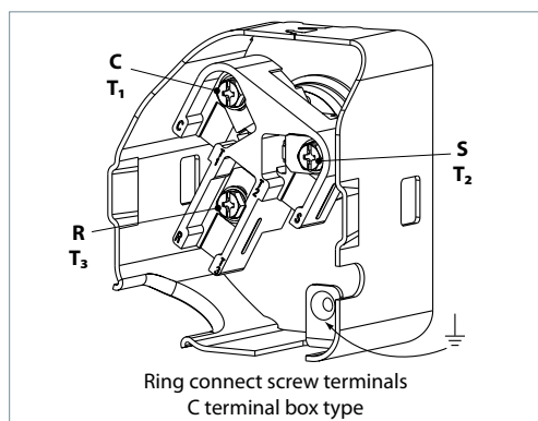
Terminal box
