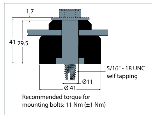
Mounting grommet
