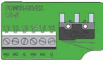
Micro switches 1, 2
